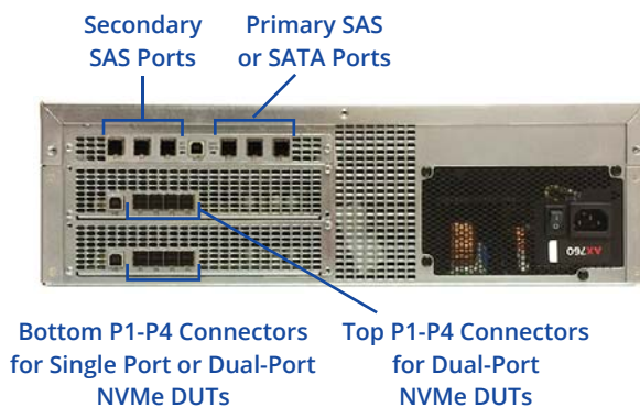
Back View of the 12-Bay U.2 Enclosure
